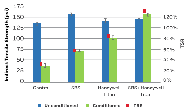
Chart 3: Tensile Strength Ratio Test (AASHTO T283)
