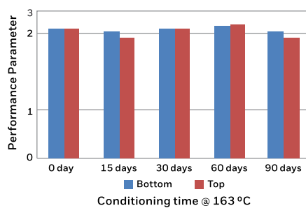
Chart 6: Storage Stability Testing (ASTM D7173)
