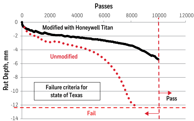
Chart 2: Results of the Hamburg Wheel test (AASHTO T324)
