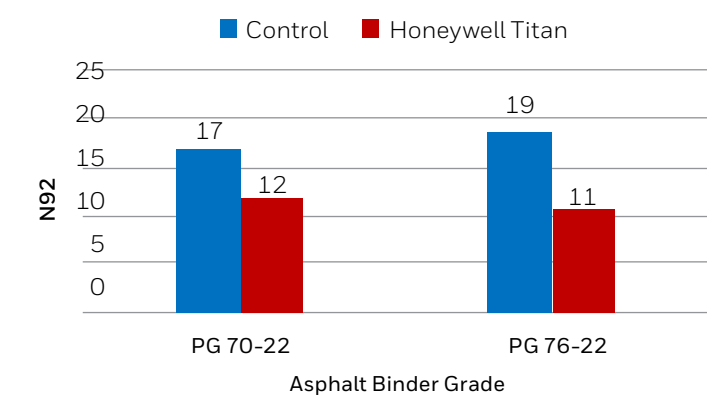
Chart 5: Number of Gyrations to achieve 92% Gmm (N92)
