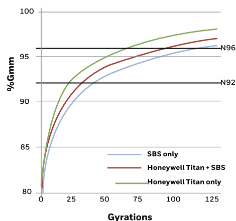
Chart 4: Compaction Benefit with Honeywell Titan
