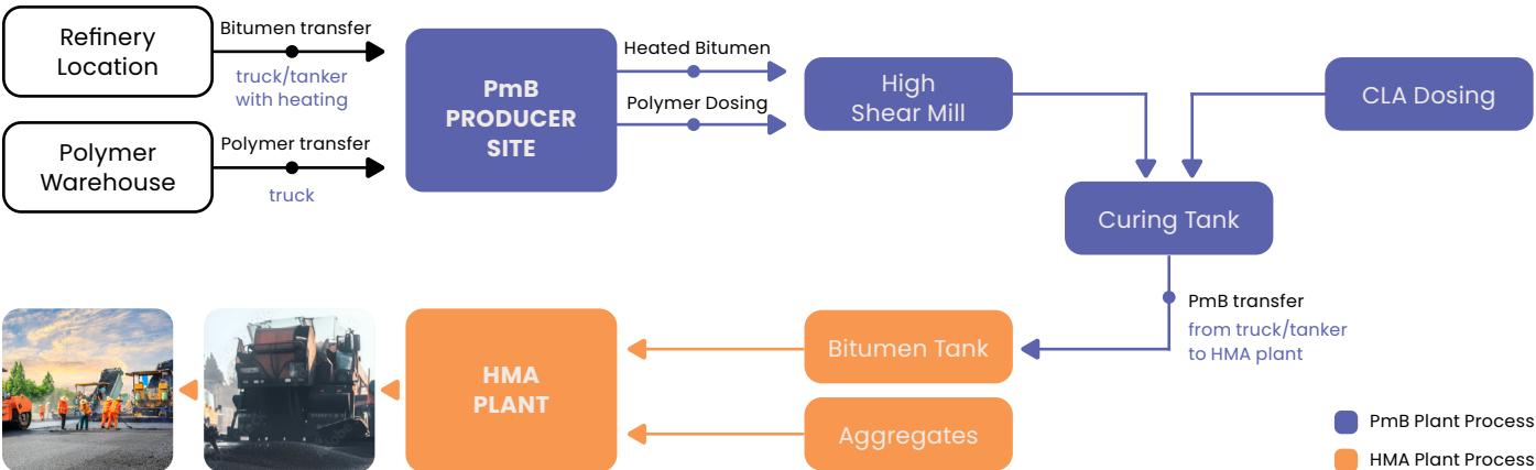
Figure 1: System boundary and stages in pavement construction process.
